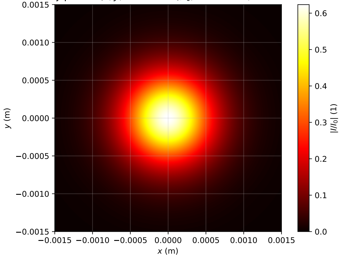
Intensity profile I(x, y, z = 3.981\text{m})/I_0 , P_{\text{in}}=0.7\text{Pcr} , artificial time
